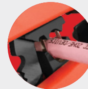
External Ground Crimp Die Properly Ground Drain Wire
