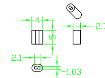
3. Wire rope's aluminum tube, red
