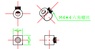
2. Hexagon screw, Black
