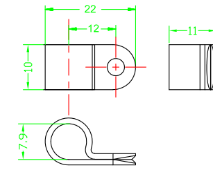
1. R Type Nylon Holder, black
