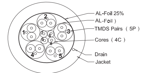
CABLE CONSTRUCTION
